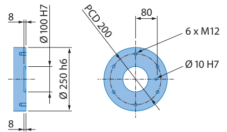
View A
