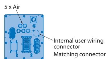
View B
