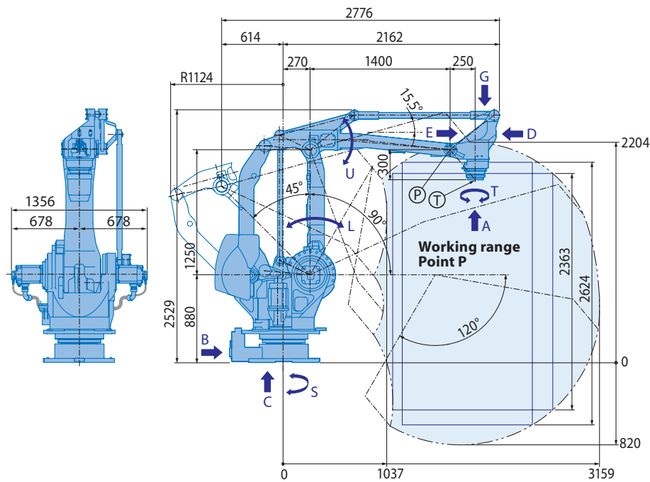
View A
